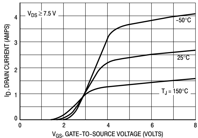
Figure 2. Transfer Function
